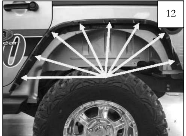
Threaded Clip locations.
